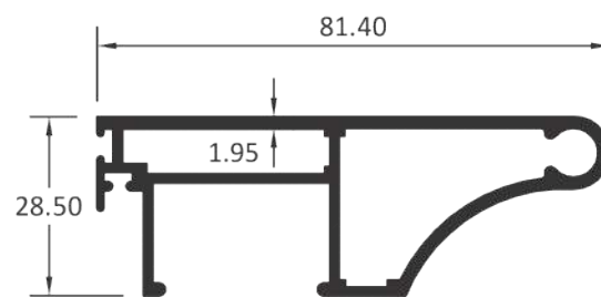
SHUTTER ADD ON
