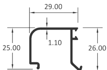
SINGLE GLASS CLIP
