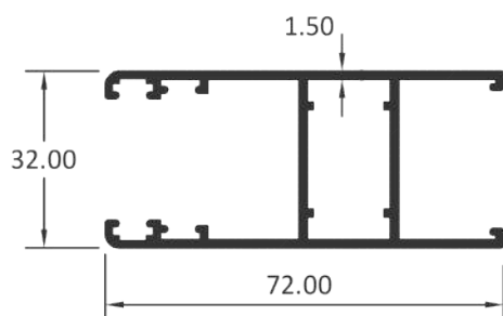
DOUBLE GLASS SHUTTER
