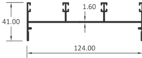
3 TRACK TOP
