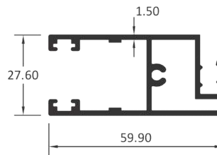
MESH SHUTTER
