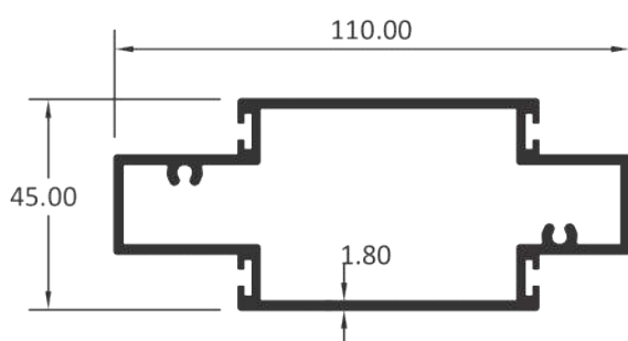
ART3007990 1.697 Kg/m
