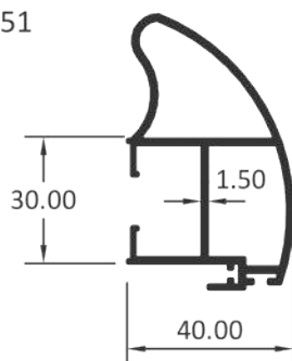
INTER LOCK ADD ON
