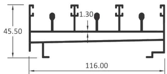
3 TRACK HOLLOW BOTTOM
