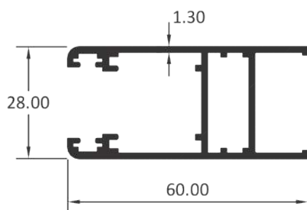
DOUBLE GLASS SHUTTER
