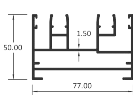
2 TRACK WITH GUIDE
