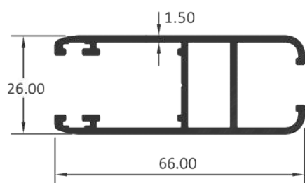
SINGLE GLASS SHUTTER
