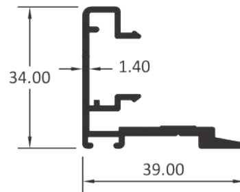
INTER LOCK CLIP
