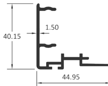
INTER LOCK CLIP
