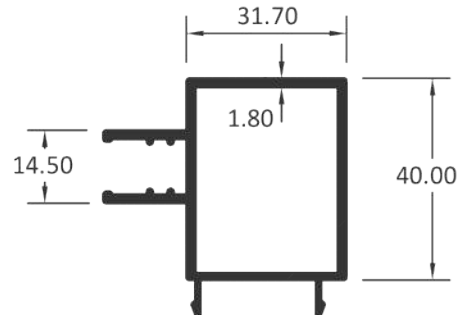
SLIDING CORNER CLIP
