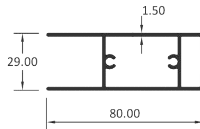
SINGLE GLASS TOP BOTTOM
