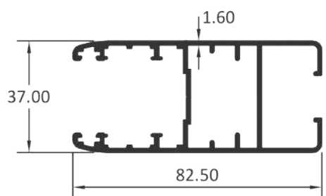
SINGLE GLASS SHUTTER
