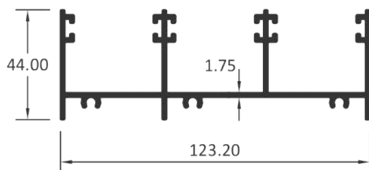
3 TRACK TOP
