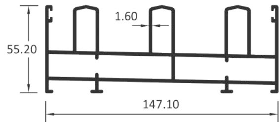
3 TRACK
