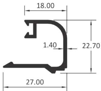
DOUBLE GLASS CLIP
