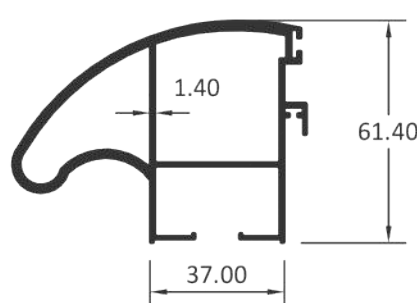
INTER LOCK ADD ON
