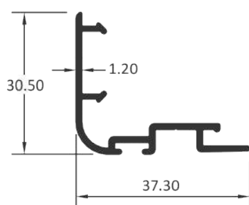
INTER LOCK CLIP
