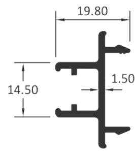
MIDDLE CLIP
