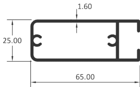
HANDLE
