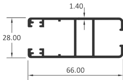
SINGLE GLASS SHUTTER
