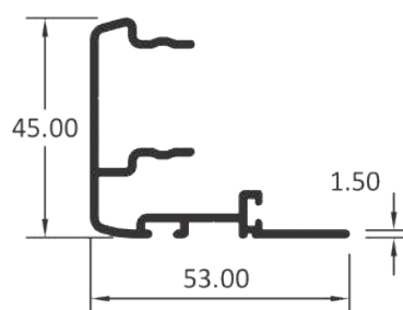
INTER LOCK CLIP
