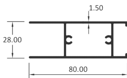
DOUBLE GLASS TOP BOTTOM
