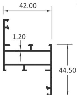
Z SHUTTER
