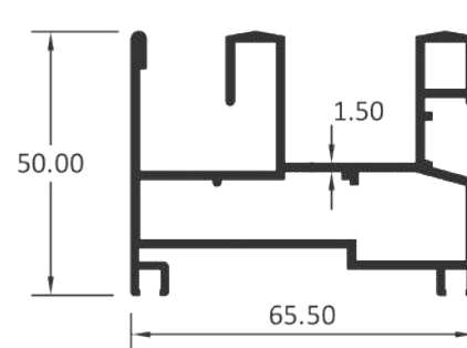
2 TRACK
