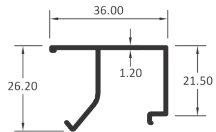
SINGLE GLASS CLIP
