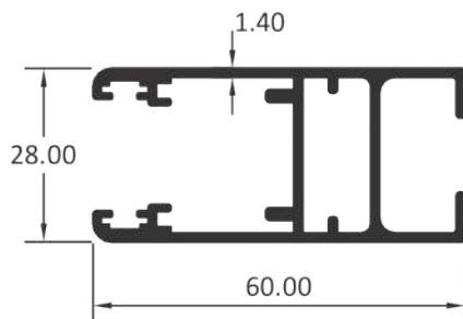
SINGLE GLASS SHUTTER
