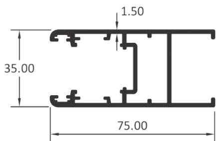
DOUBLE GLASS SHUTTER
