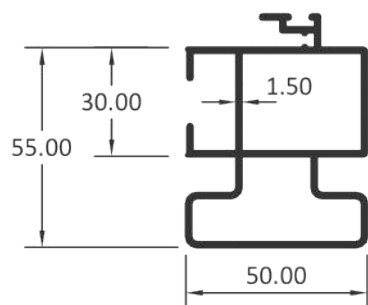
INTER LOCK ADD ON
