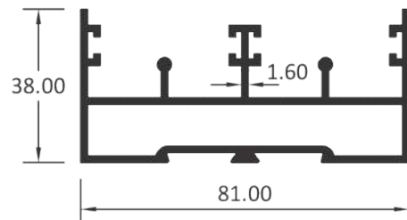
2 TRACK HOLLOW BOTTOM
