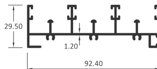
3 TRACK BOTTOM
