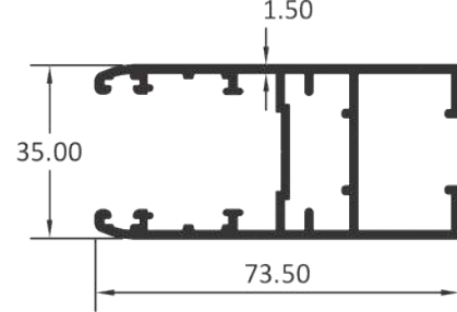
SINGLE GLASS SHUTTER
