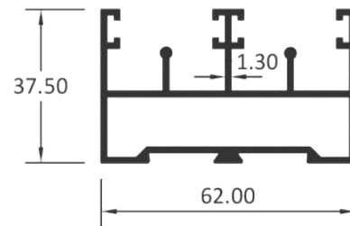
2 TRACK HOLLOW BOTTOM
