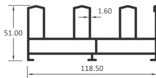
3 TRACK
