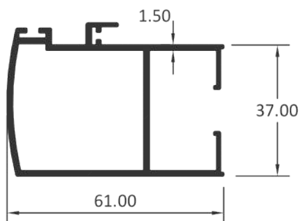
INTER LOCK
