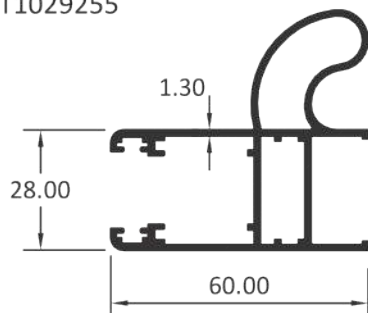
DOUBLE GLASS SHUTTER ADD ON
