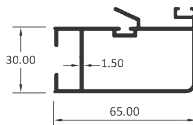
SINGLE GLASS INTER LOCK
