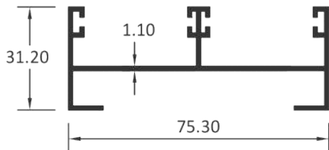
2 TRACK TOP
