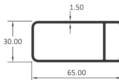
DOUBLE GLASS HANDLE
