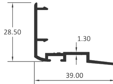
INTER LOCK CLIP
