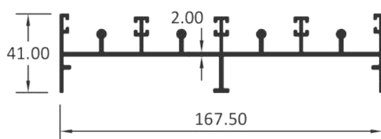
4 TRACK BOTTOM
