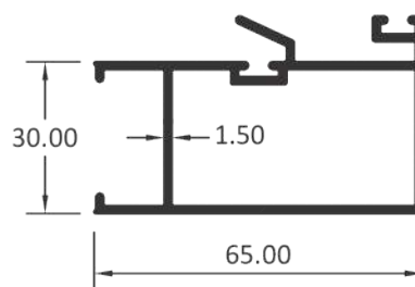
DOUBLE GLASS INTER LOCK
