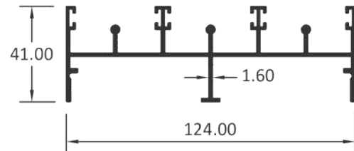
3 TRACK BOTTOM
