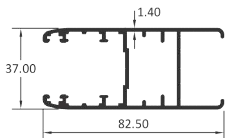
DOUBLE GLASS SHUTTER
