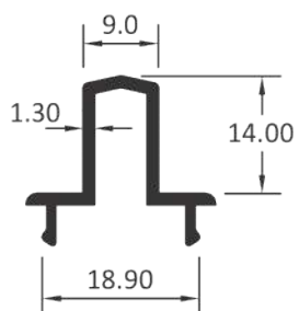
MIDDLE CLIP
