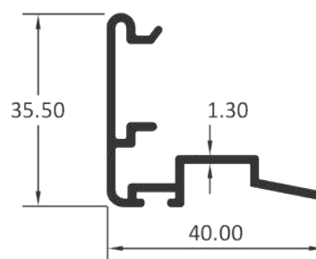
INTER LOCK CLIP
