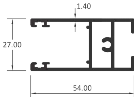
SHUTTER
