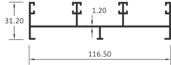
3 TRACK TOP
