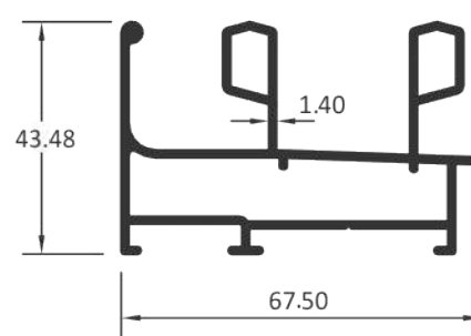
2 TRACK
