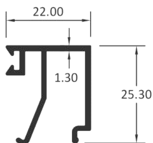
DOUBLE GLASS CLIP
