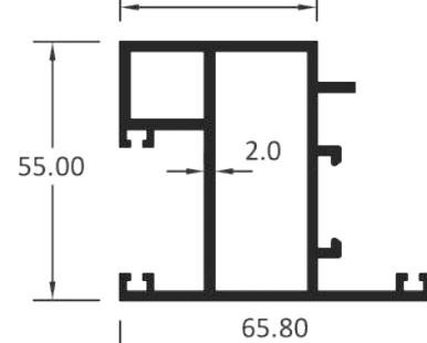
L CORNER MULLION
