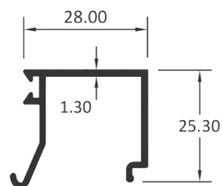
SINGLE GLASS CLIP
