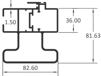
INTER LOCK SHUTTER ADD ON
