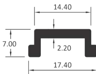
SLIDING BAR
