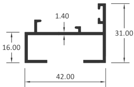
FRAME
