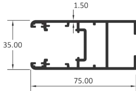
SINGLE GLASS SHUTTER
