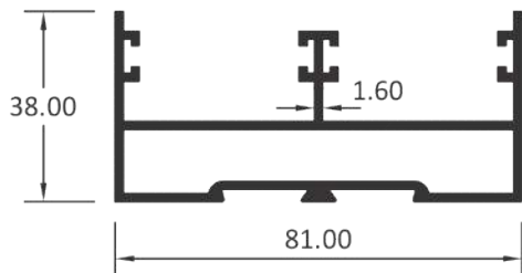
2 TRACK HOLLOW TOP
