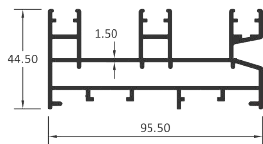
3 TRACK
