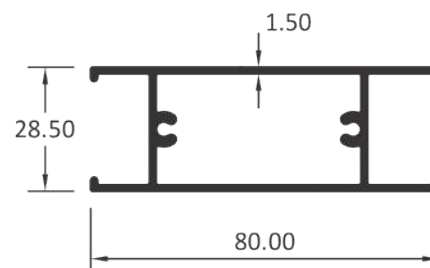
DOUBLE GLASS TOP BOTTOM
