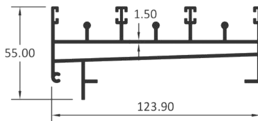
3 TRACK HOLLOW BOTTOM
