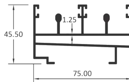
2 TRACK HOLLOW BOTTOM
