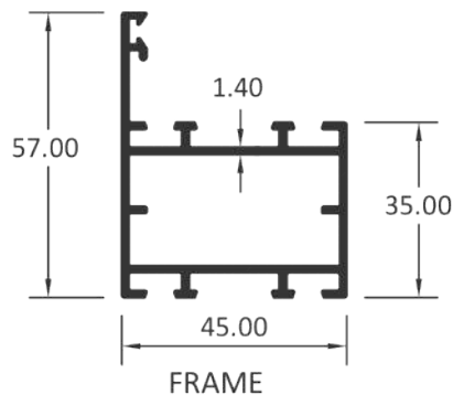
FRAME
