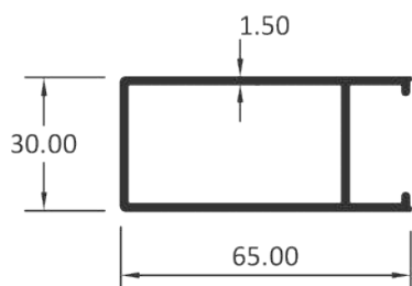
DOUBLE GLASS HANDLE
