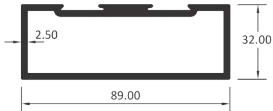
SINGLE PARTITION
