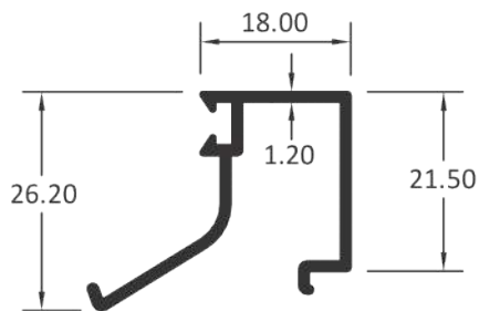
DOUBLE GLASS CLIP
