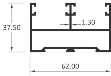
2 TRACK HOLLOW TOP
