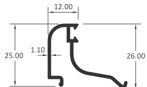
DOUBLE GLASS CLIP
