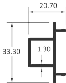
MIDDLE CLIP
